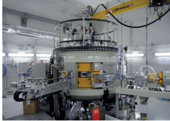
IBA Cyclone® 30 with 3 beam transport lines installed at the KFSHRC in Riyadh, KSA.
